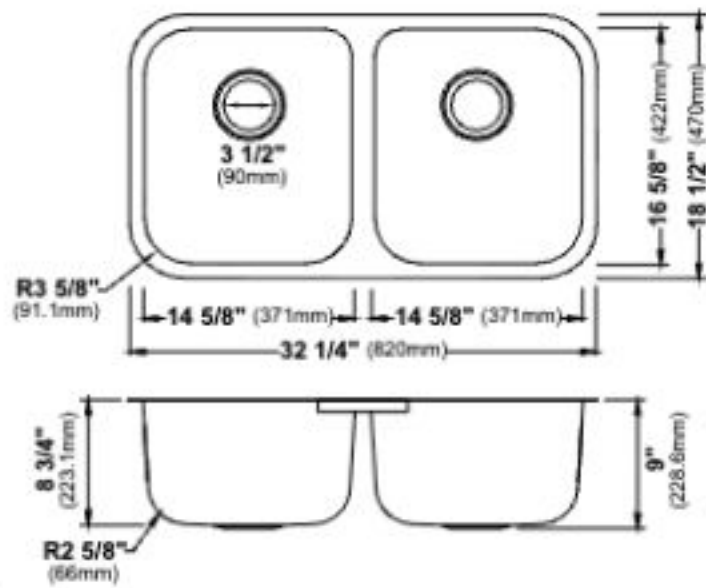
MODEL: PRU31 Stainless Steel Undermount Double Bowl Kitchen Sink
