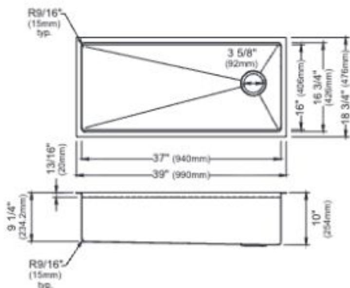
MODEL: WS-39-PK1 Stainless Steel Undermount Large Single Bowl Workstation Sink
