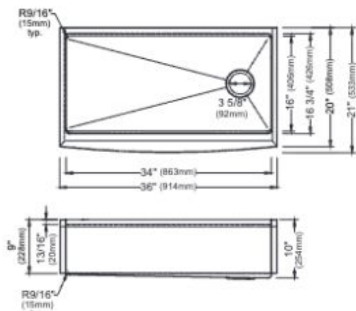
MODEL: WSA-46-PK1 Stainless Steel Large Single Bowl Apron Front Sink
