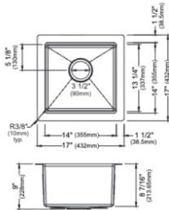
MODEL: HSU1717SB Matrix Steel Undermount Single Bowl Workstation Bar Sink
