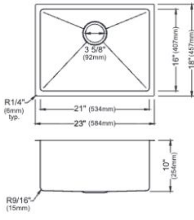
MODEL: EL-73-PK1 Stainless Steel Undermount Single Bowl Kitchen Sink
