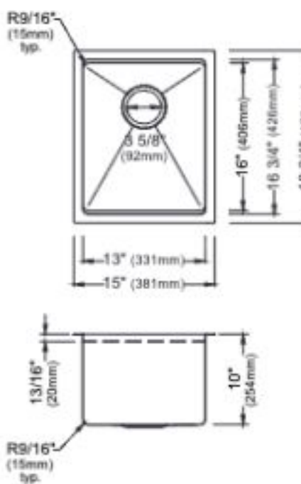
MODEL: WS-31-PK1 Stainless Steel Undermount Single Bowl Workstation Bar Sink
