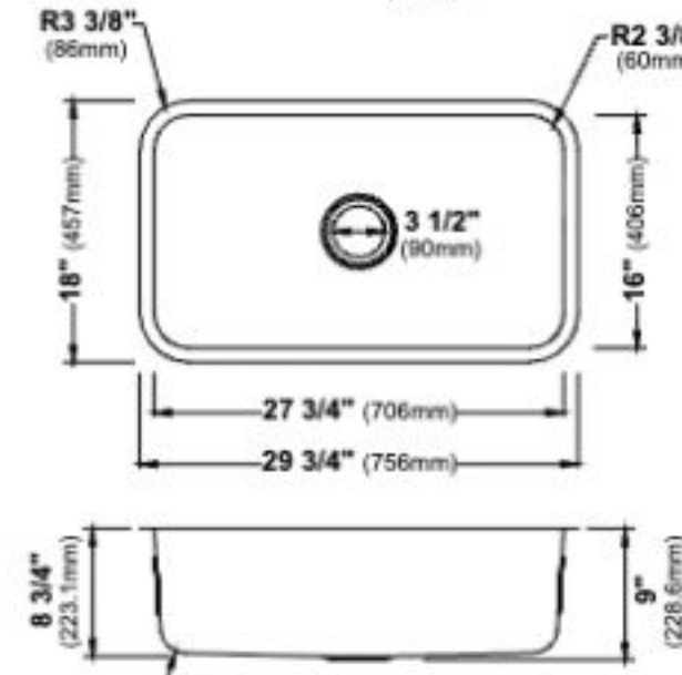
MODEL: PRU35 Stainless Steel Undermount Large Single Bowl Kitchen Sink
