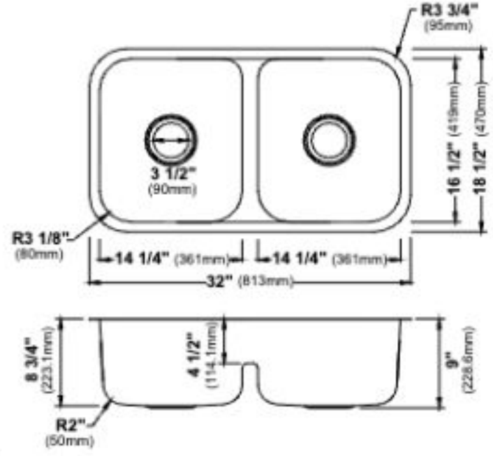
MODEL: PRU32 Stainless Steel Undermount Double Bowl Kitchen Sink
