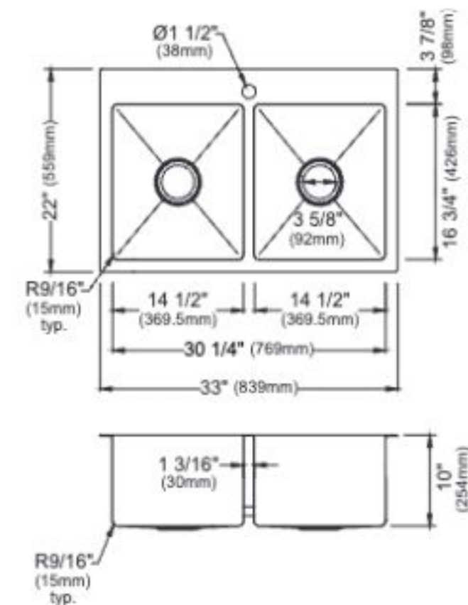
MODEL: EL-35-PK1 Stainless Steel Top Mount Double Bowl Kitchen Sink
